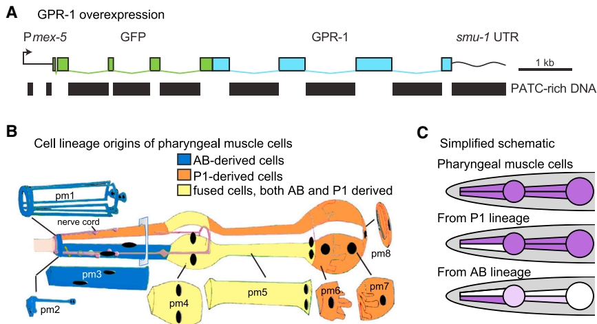
(C) Simplified schematic of fluorescently expressing AB, P1, and fused cells as viewed under a dissection microscope. Note that the fluorescence intensity in fused cells depends on the proportion of nuclei from the AB versus P1 lineage. For example, in the AB-derived pattern, expression is limited to 1/6 nuclei in PM4 and 2/6 nuclei in PM5, resulting in partial expression and dim fluorescence. The fainter fluorescence in these compartments can be difficult to visualize. Also, PM1 is not indicated in the schematic, as it is hard to observe at low-magnification fluorescence microscopy.
