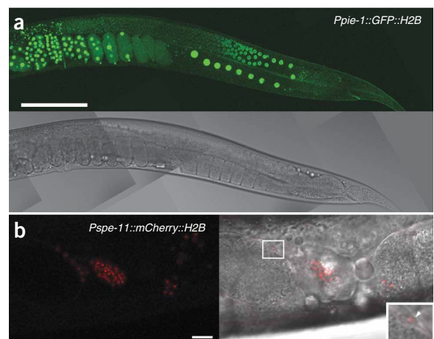
Figure 4 MosSCI inserts are expressed in the female and male germlines. (a) The Ppie-1::GFP::H2B transgene was expressed throughout the female germline. Scale bar = 100 \mu m. (b) The Pspe-11::mCherry::H2B transgene was expressed in hermaphrodite sperm. Left, mCherry expression from Pspe-11::mCherry::H2B was specific to hermaphrodite sperm. Scale bar = 10 \mu m. Right, overlay with differential interference contrast image. Most sperm were found in the spermatheca, although a few were also seen in the gonad and uterus. Right inset shows larger view of boxed area, in which mCherry expression is localized to nucleus (arrowhead). Magnification, \times 4 .
